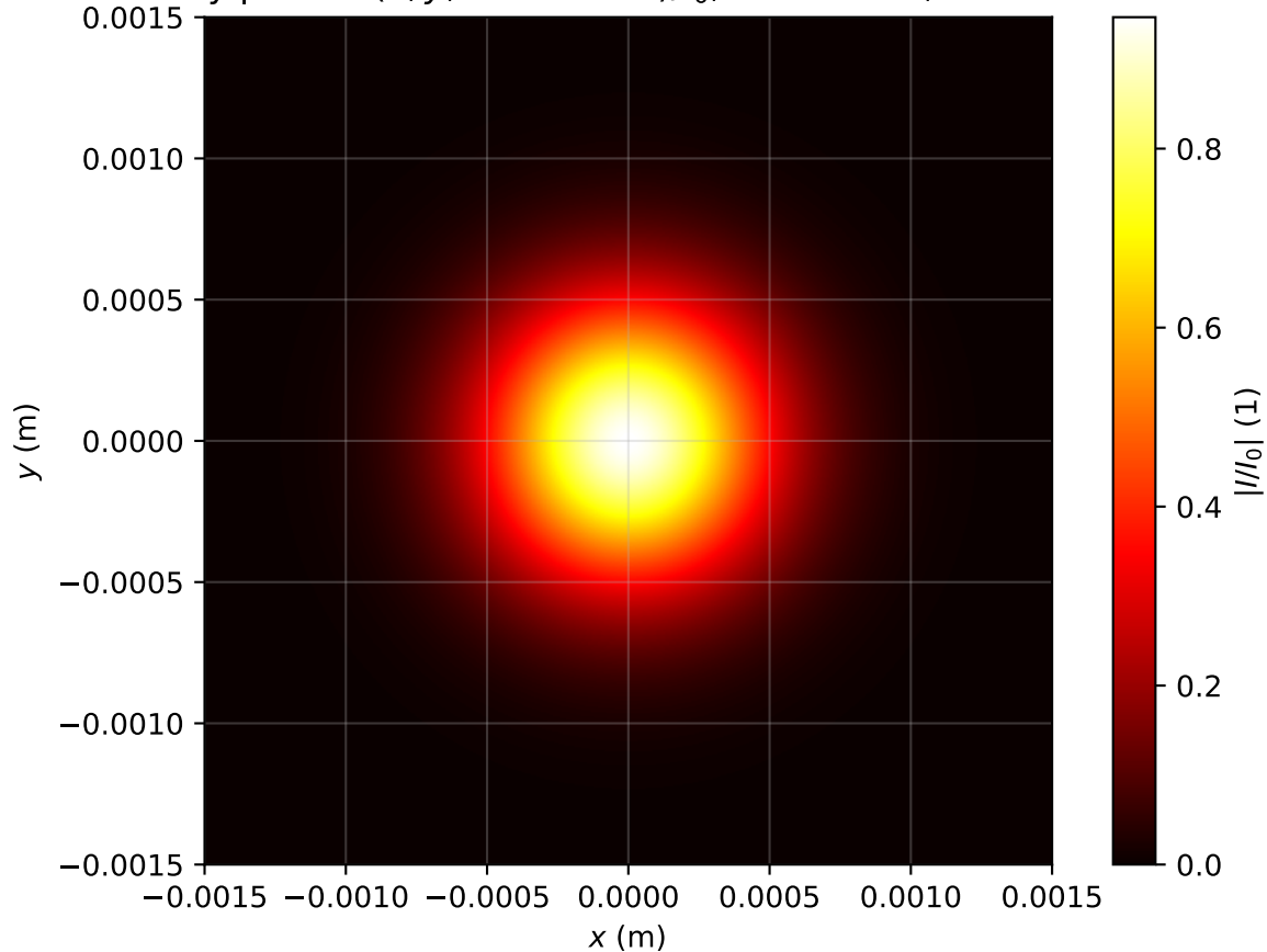
Intensity profile I(x, y, z = 0.716m)/I_0 , Pin=0.2Pcr, artificial time
